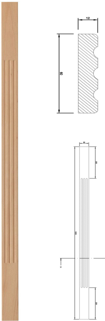
CP6012120/60x12x1200 mm
