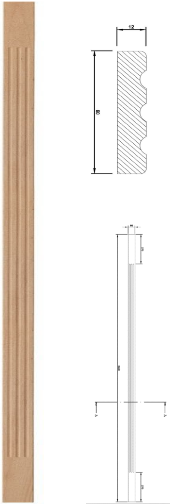
CP6012240/60x12x2440 mm
