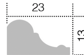
L8040MD/23*13*2440 mm
