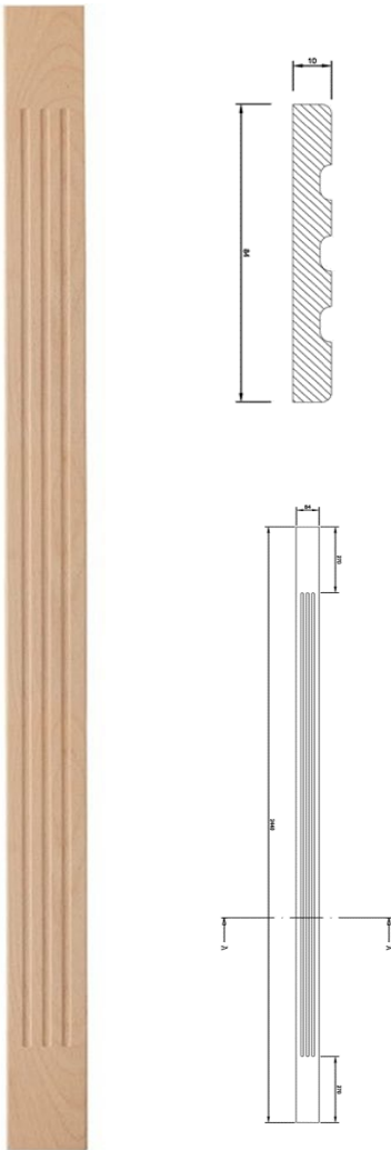
CP8410240/84x10x2440mm
